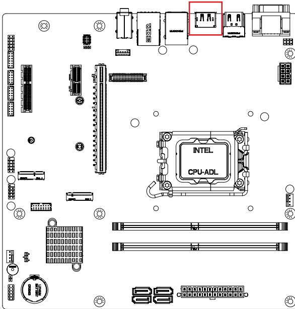
DP Connector
